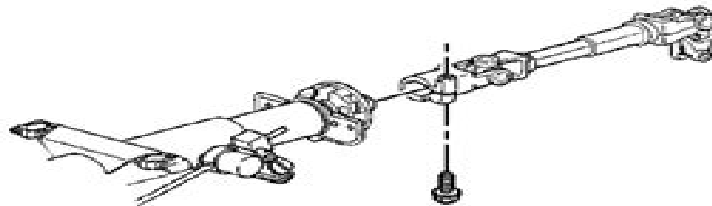
Fig. 11: View Of Upper Pinch Bolt Of Intermediate Steering Shaft Courtesy of GENERAL MOTORS CORP.
