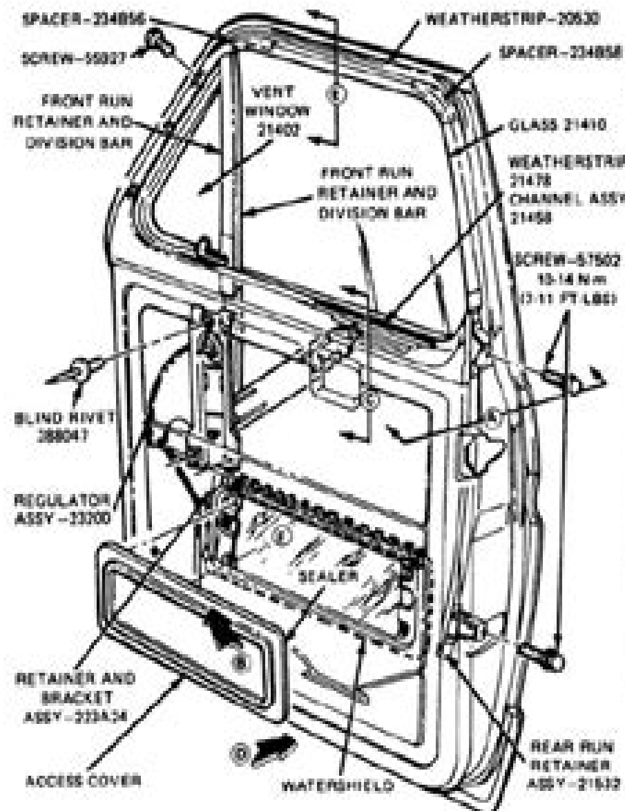
FIG : Fig. 4 Exploded view of the front window glass and regulator mounting-1979-88 models
