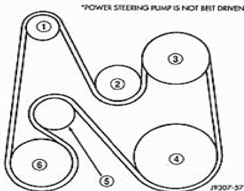
Fig. 21 Belt Routing—5.9L Diesel Engine—With A/C
