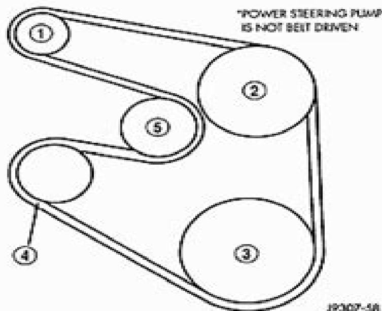
Fig. 22 Belt Routing—5.9L Diesel Engine—Without A/C
