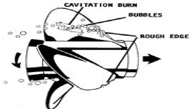
Cavitation (air bubbles) formed at the propeller. Manufacturers are constantly fighting this problem, as explained in the text.
