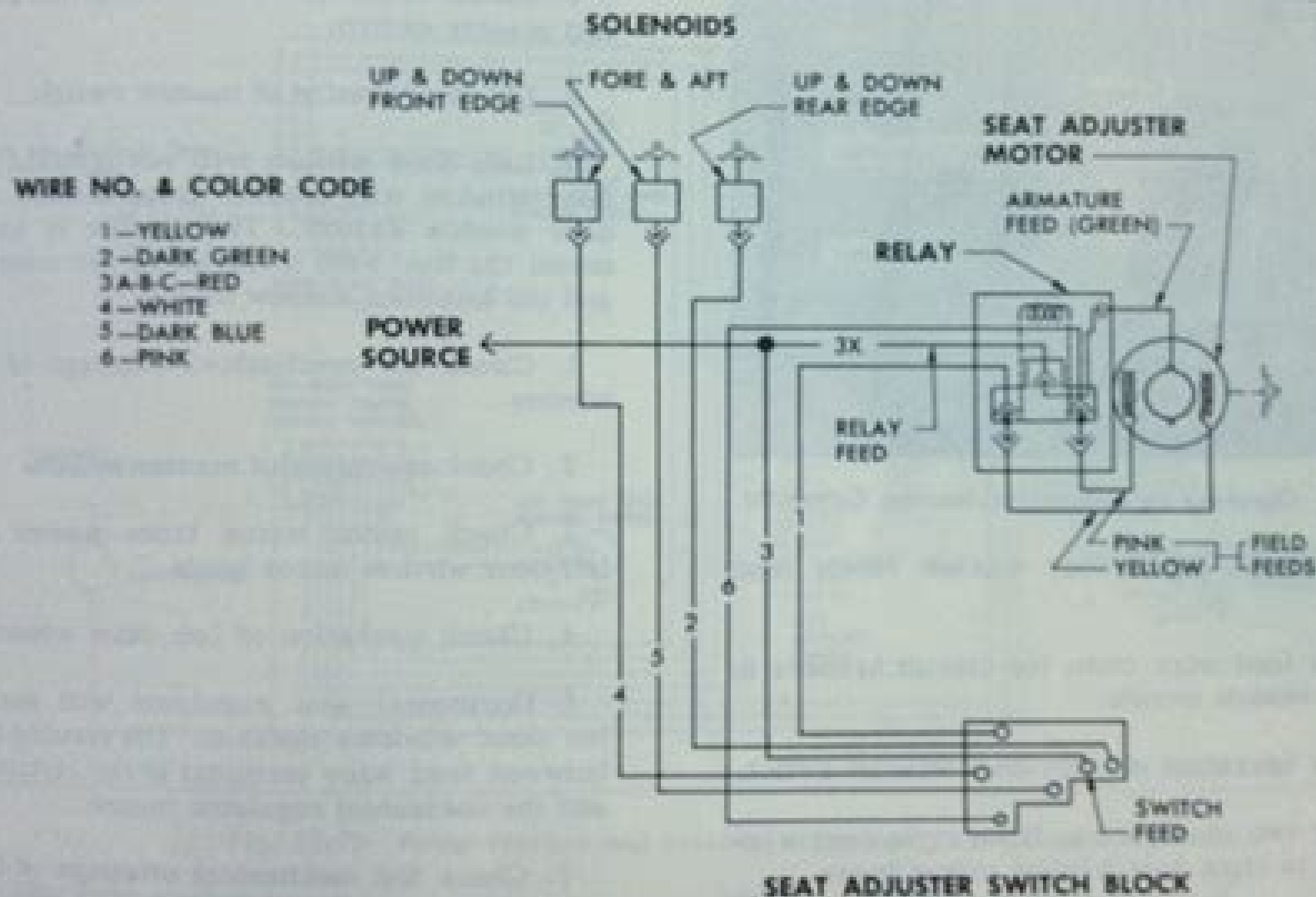
Fig. 17-74 Six-Way Seat Circuit Diagram
