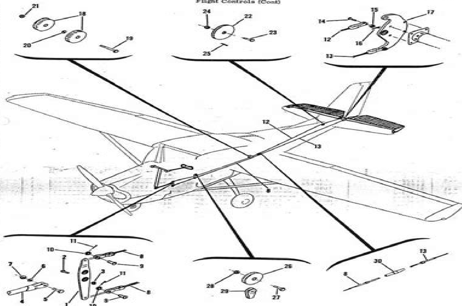
Figure 154. Elevator Control System Installation
