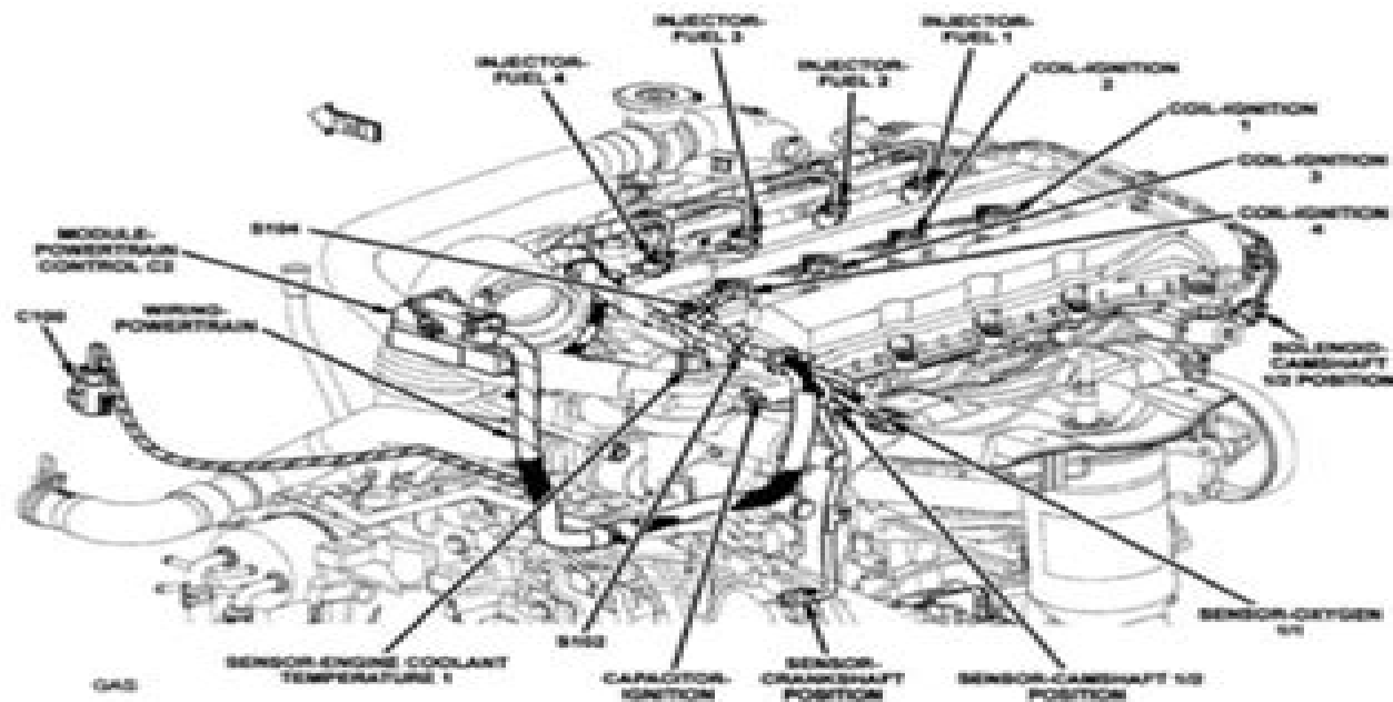
Fig. 17: Left Rear Of Engine Courtesy of CHRYSLER LLC
