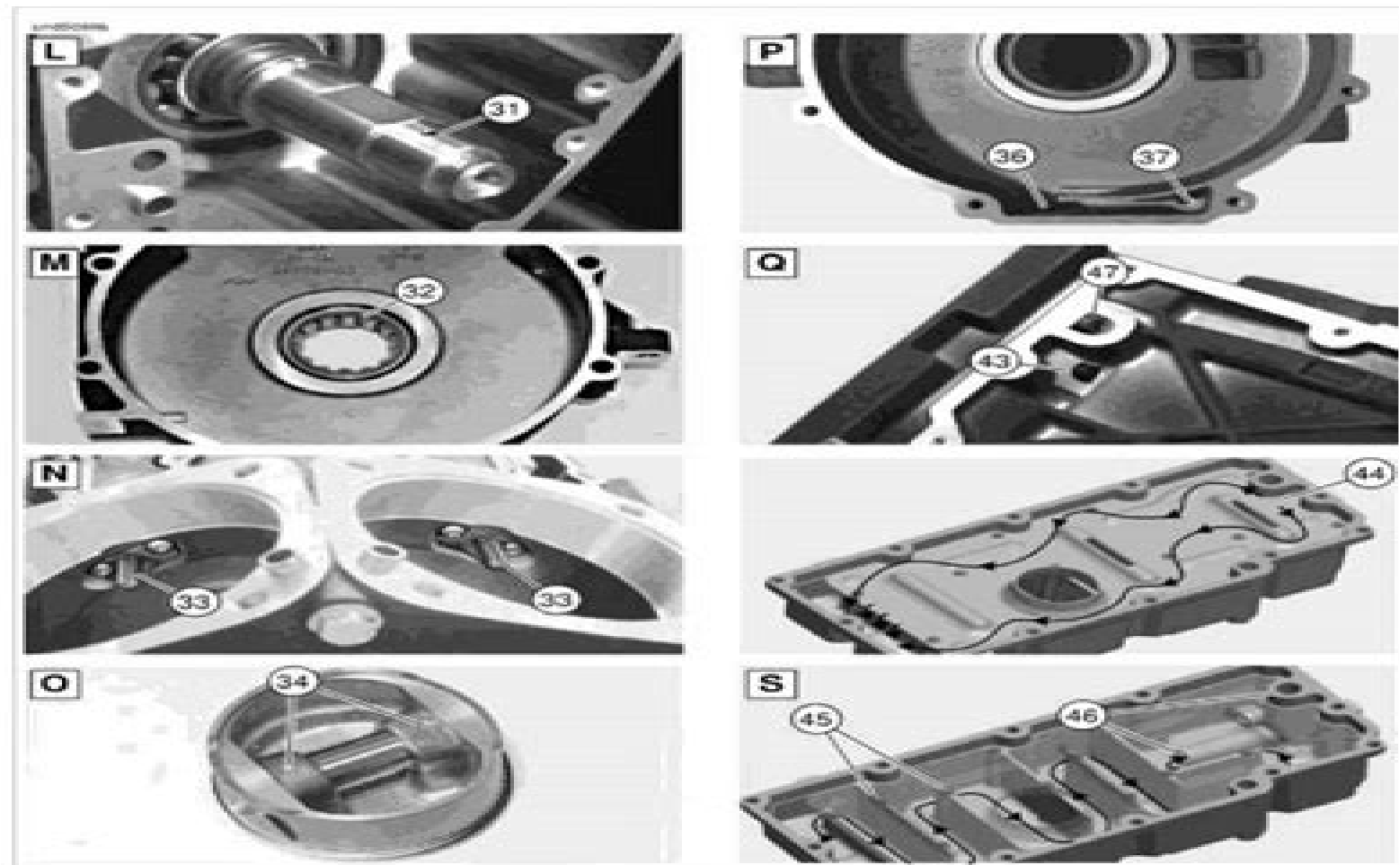
Figure 3-3. Engine Oil Flow - Bottom End
