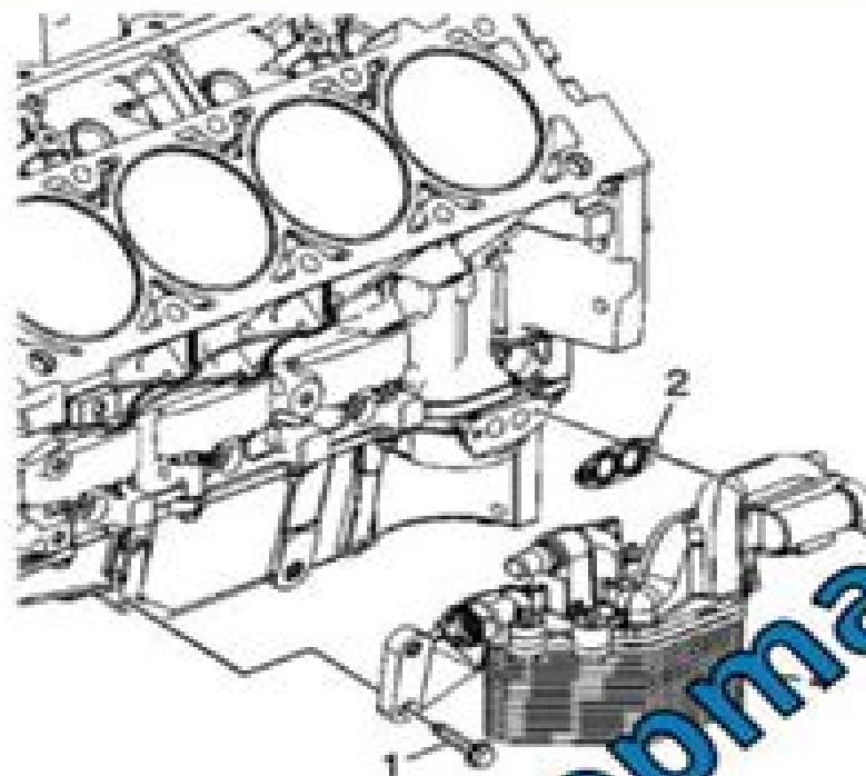
Fig. 105: Identifying Oil Cooler Components Courtesy of GENERAL MOTORS
