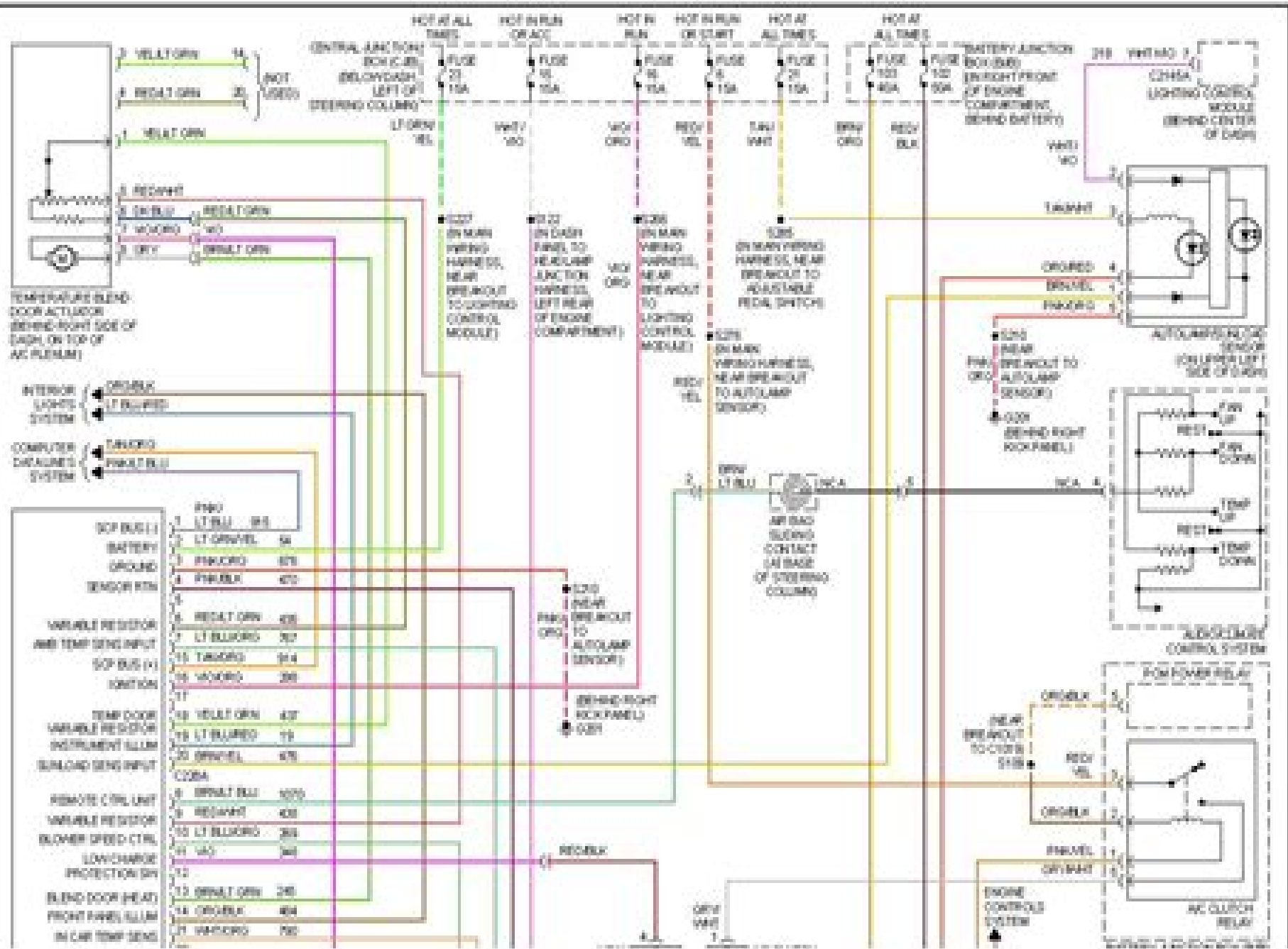
2004 Ford Crown Victoria-Fig. 1: Automatic A/C Circuit
