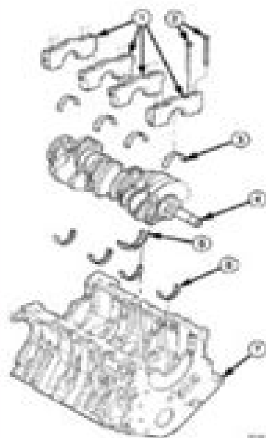
Fig. 347: Cylinder Block & Crankshaft Courtesy of CHRYSLER LLC
