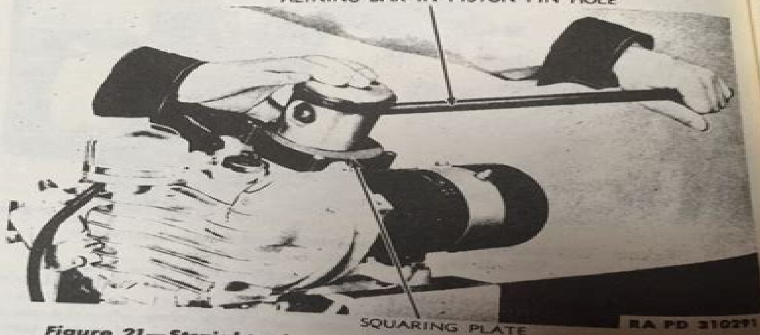
ALINING BAR IN PISTON PIN HOLE
