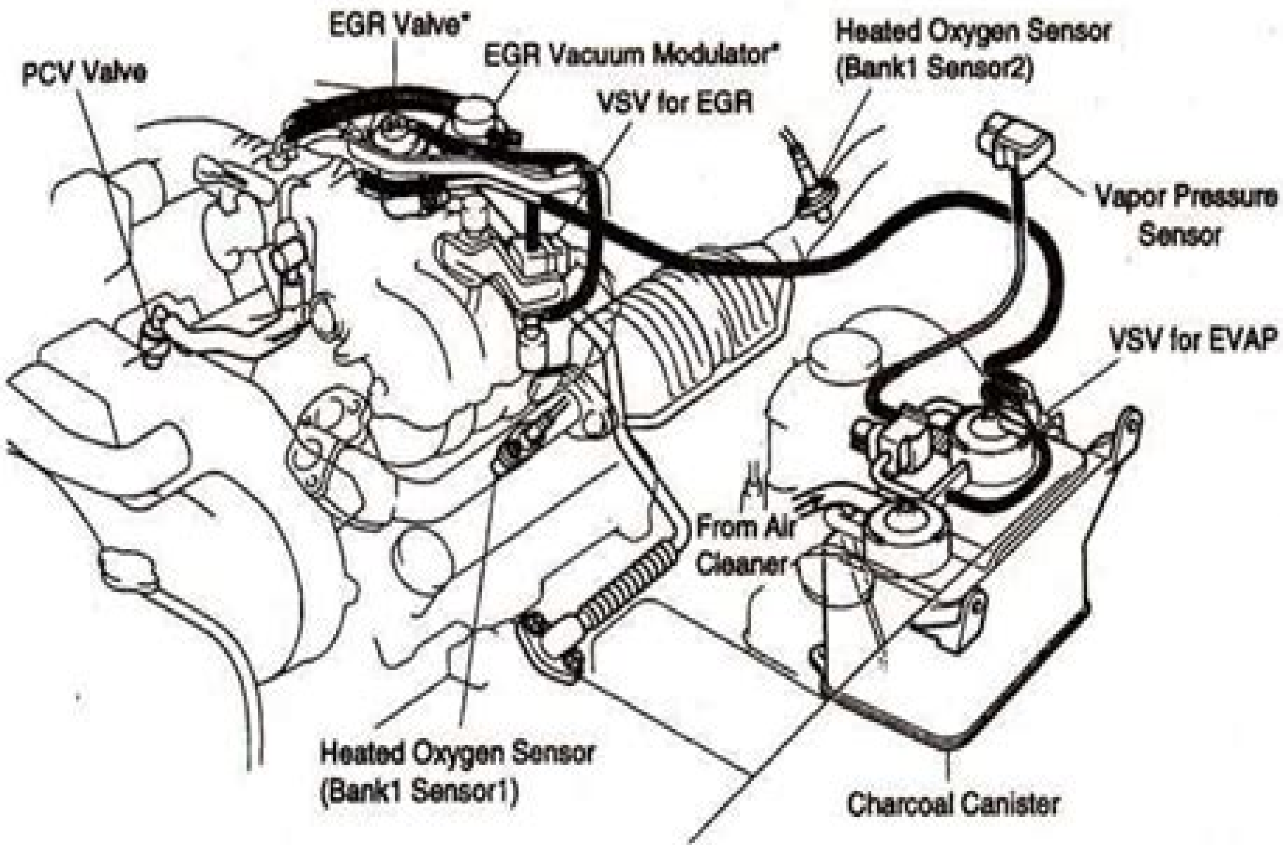
1.3c Vacuum hose routing diagram - 3.4L V6 engine
