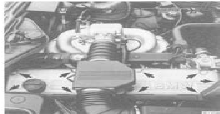
Fig. 6. Cylinder head cover fasteners (arrows).
