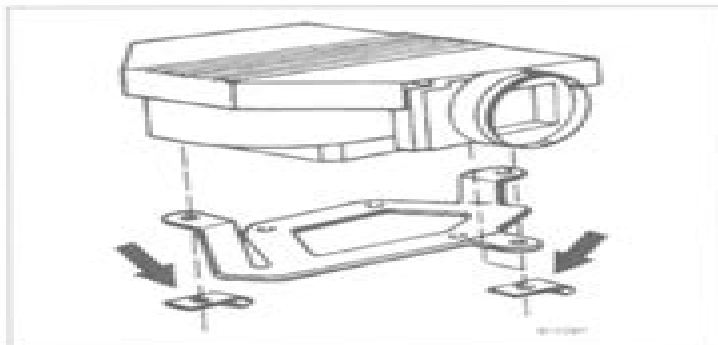
Fig. 5. Air flow sensor mounting clips on M50 engine (arrows).
