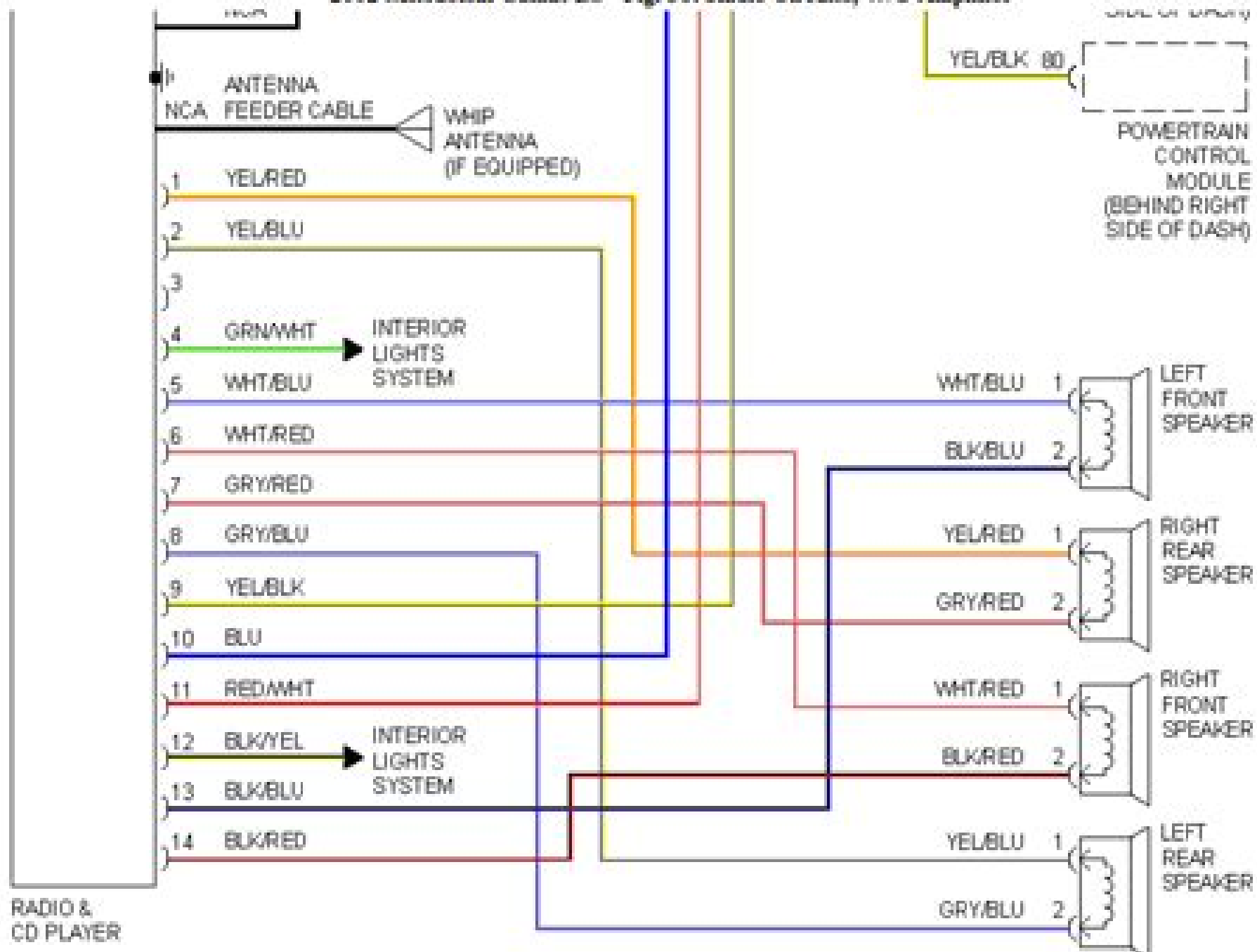
2002 Mitsubishi Galant ES - Fig. 36: Radio Circuits, W/O Amplifier
