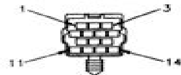
OEM INTERFACE CONNECTOR 14 PIN CONNECTOR*
