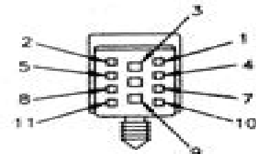
OEM INTERFACE CONNECTOR 11 PIN CONNECTOR*
