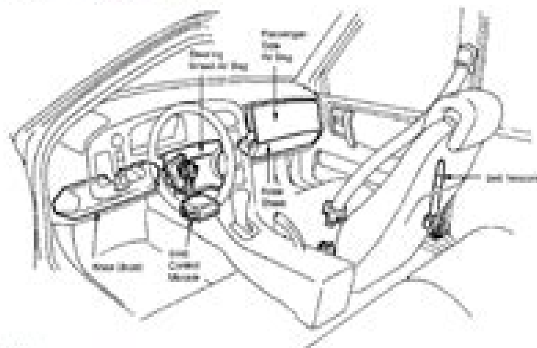
Fig. 1: Locating SRS Components Courtesy of Saab-Scania of America, Inc.
