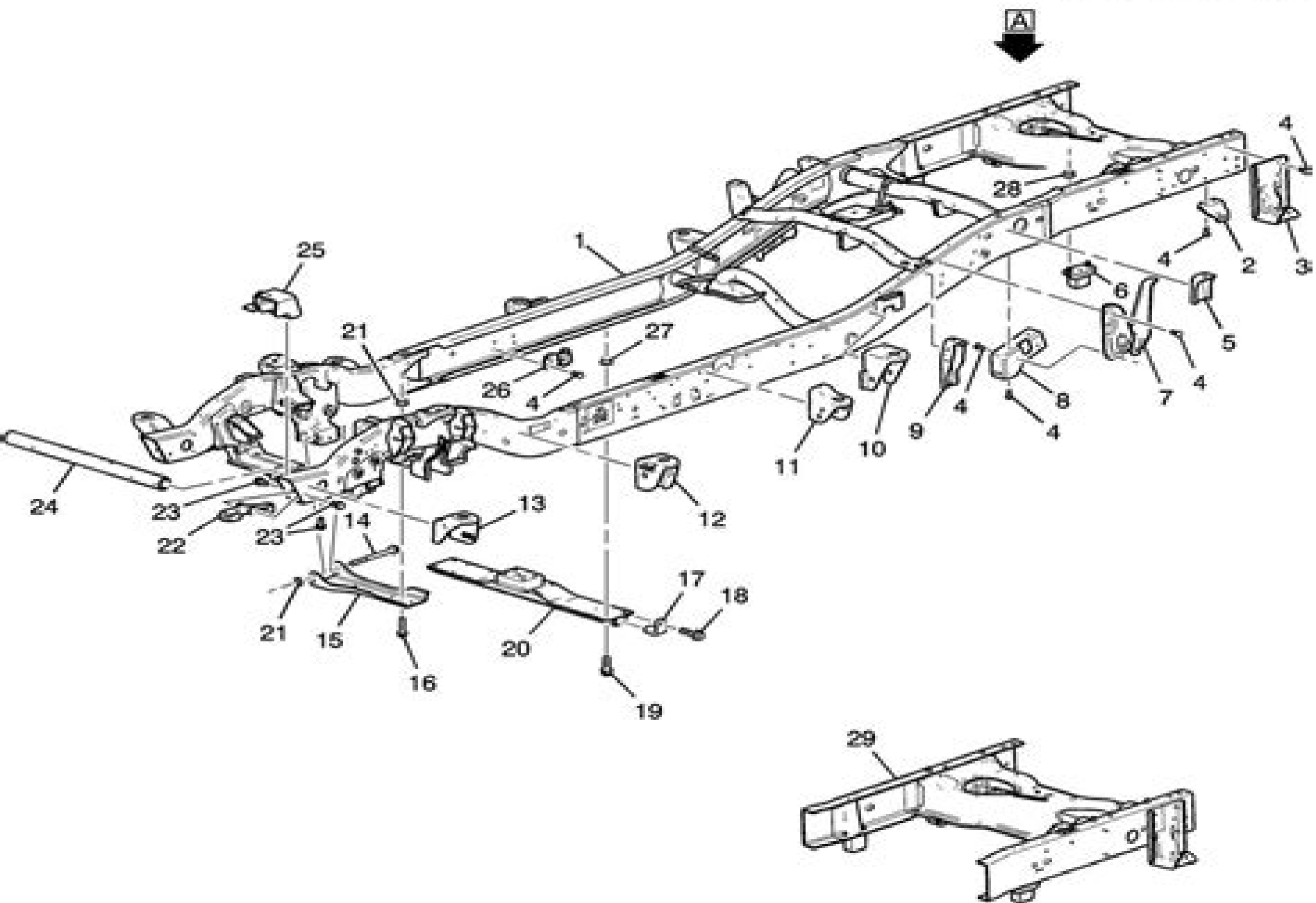
VIEW A
