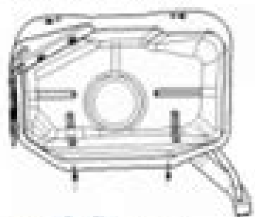
4.2.12 Remove 3 bolts and fuel tank vent hose.
