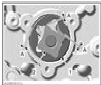
1. Inner rotor 2. Outer rotor 3. Oil pump shaft 4. Needle pin
