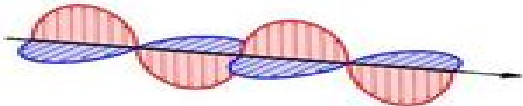
Electromagnetic Wave
