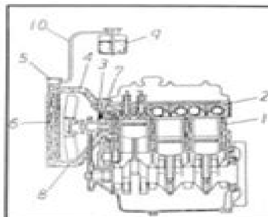
FIGURE 8 - Cooling System Schematic Diagram
