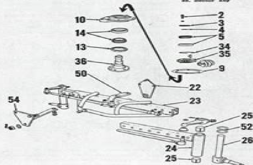
Fig. AC7—Models WD and WD-45 adjustable axle version main steering gear, and axle assembly.
