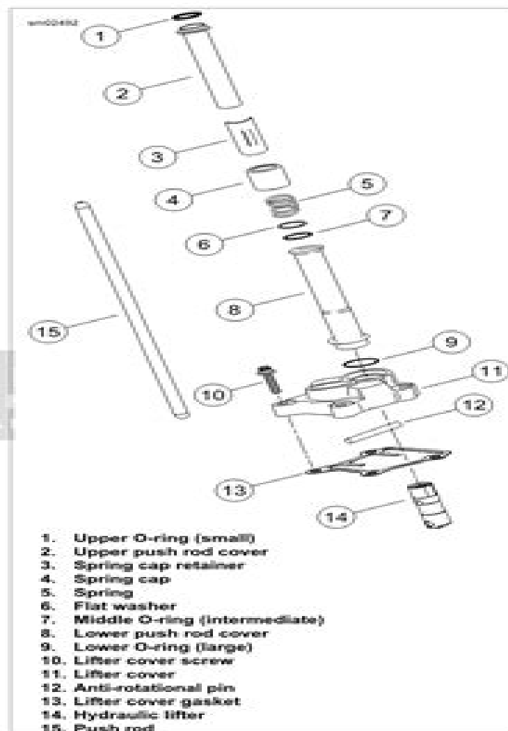
Figure 3-78. Push Rods, Lifters and Covers
