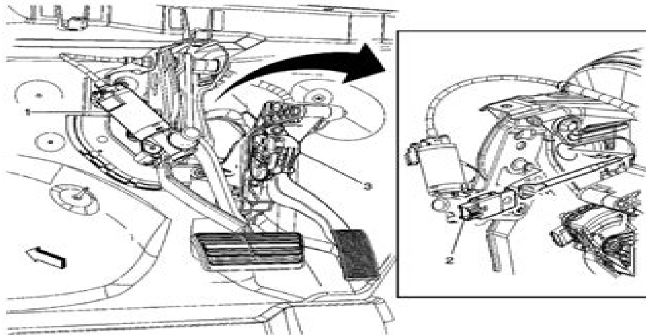
Fig. 3: Pedal Assemblies
