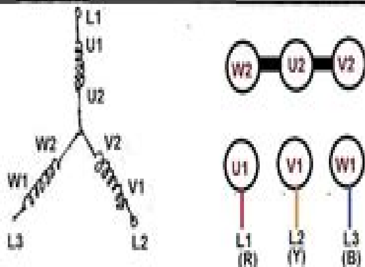
(1) STAR CONNECTION ( 6 LEADS)
