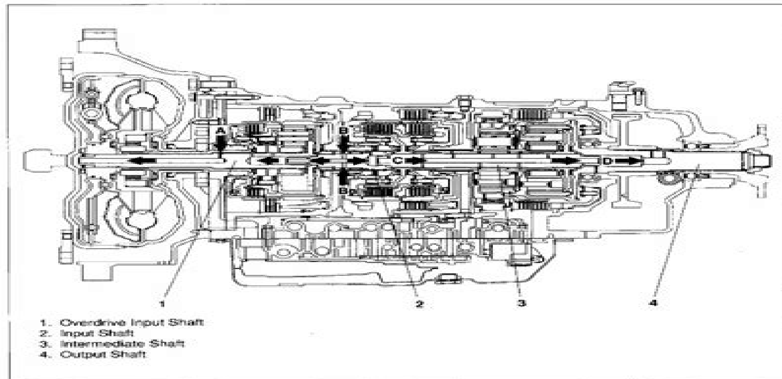
Figure 6. Shaft
