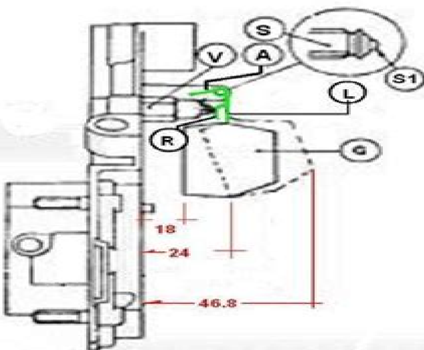
DGV Series w/Plastic Float
