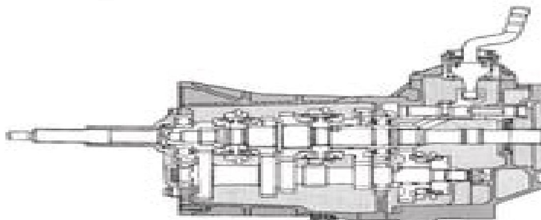
Fig. 1 AX 4/5 Manual Transmission
