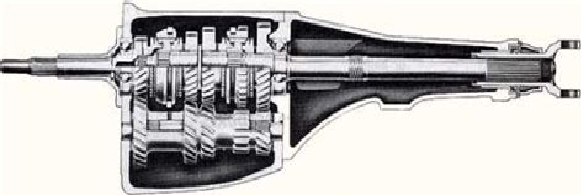
Fig. 1 - A-833 Four Speed Transmission - Cross Section
