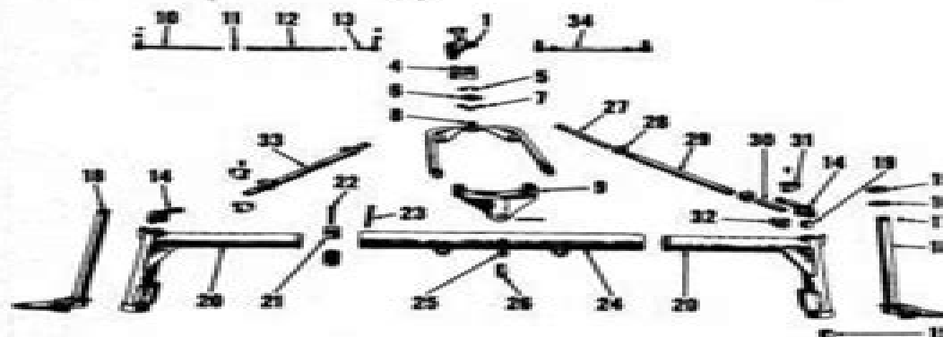
Fig. 6-Expanded view of adjustable wide front axle used on Farmall "Hi-Clear" models. Note the auxiliary stay rod assemblies.
