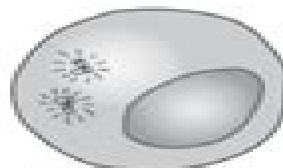
Prophase I
