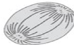
Anaphase II
