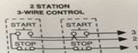
2-STATION 3-WIRE CONTROL
