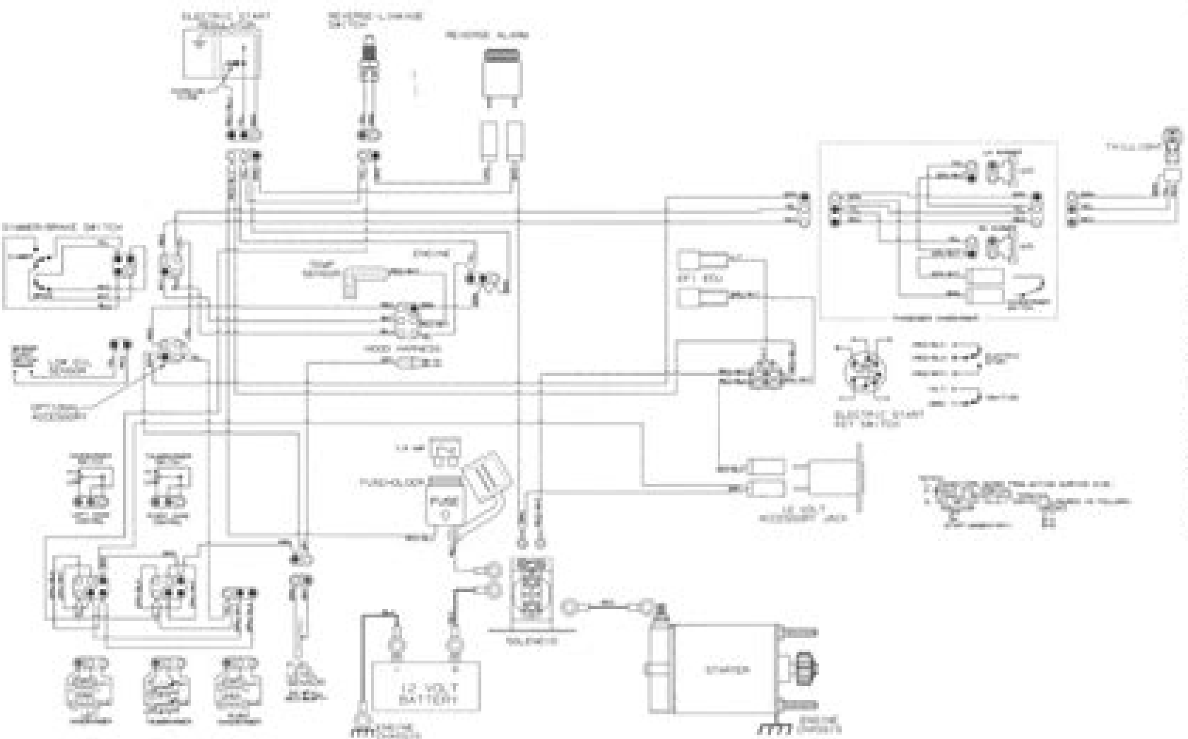
WINDING DIAGRAM
