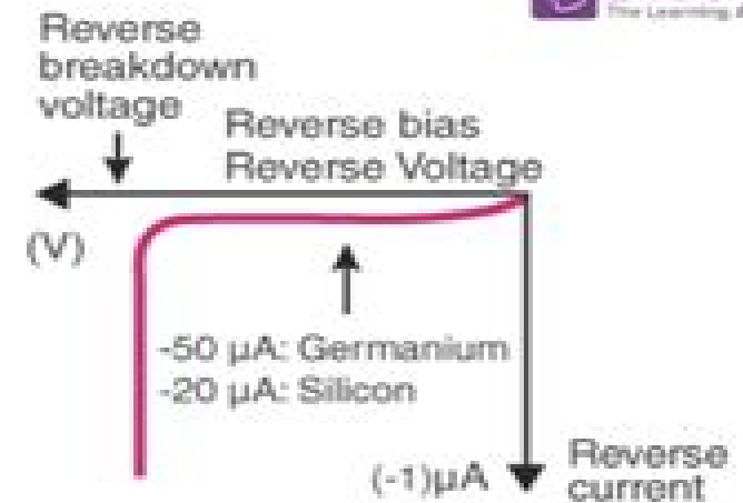
Reverse-biased diode
