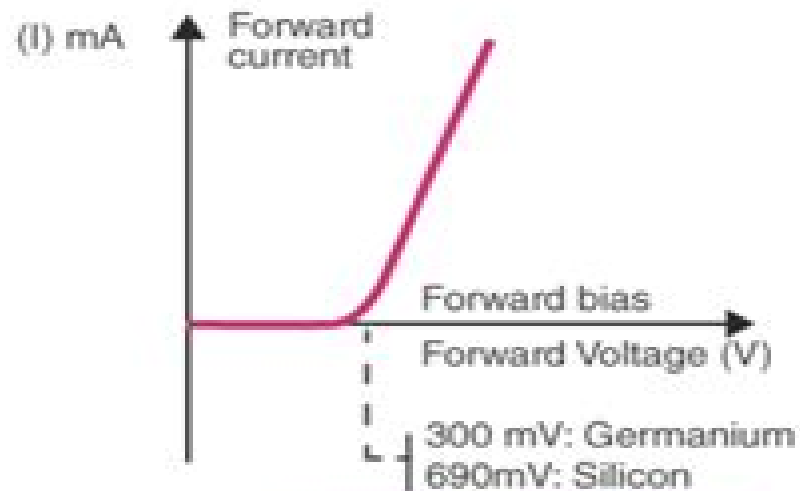
Forward-biased diode
