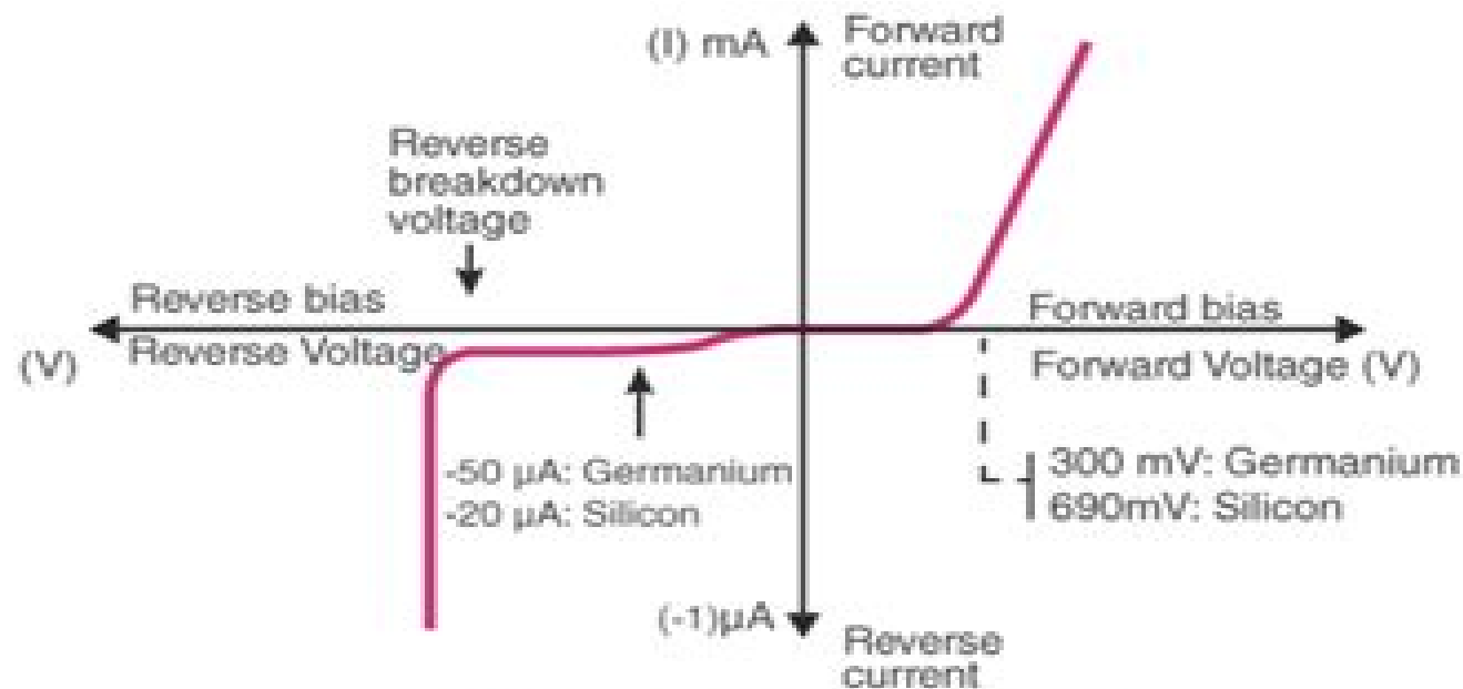
VI characteristics of Diode
