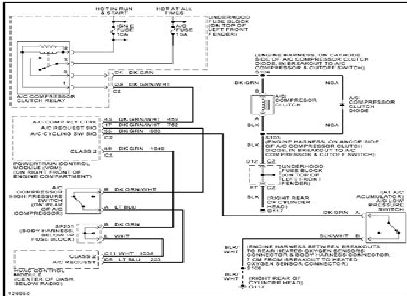
Fig. 2: Compressor Circuit, Auto A/C
