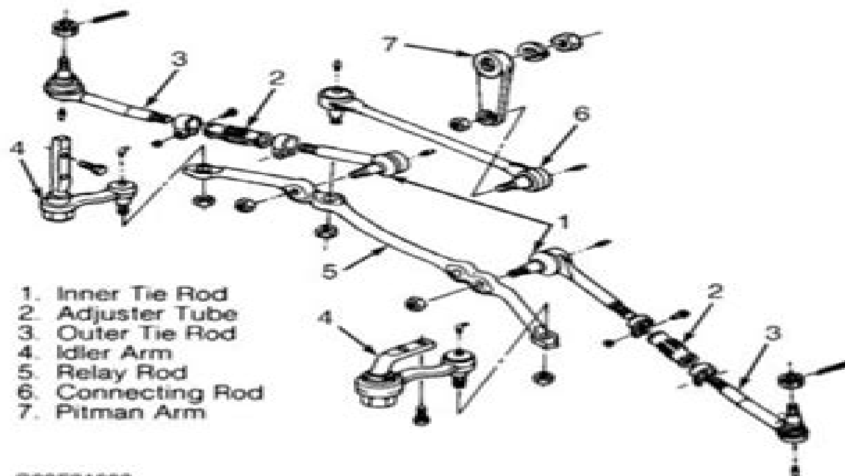
Fig. 2: Exploded View Of Steering Linkage (Astro & Safari - 2WD) Courtesy of GENERAL MOTORS CORP.
