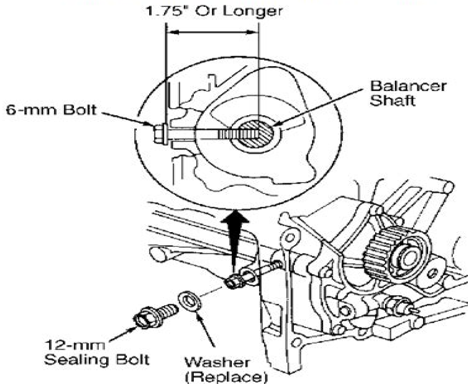
Fig. 6: Installing Balancer Shaft Lock Bolt
