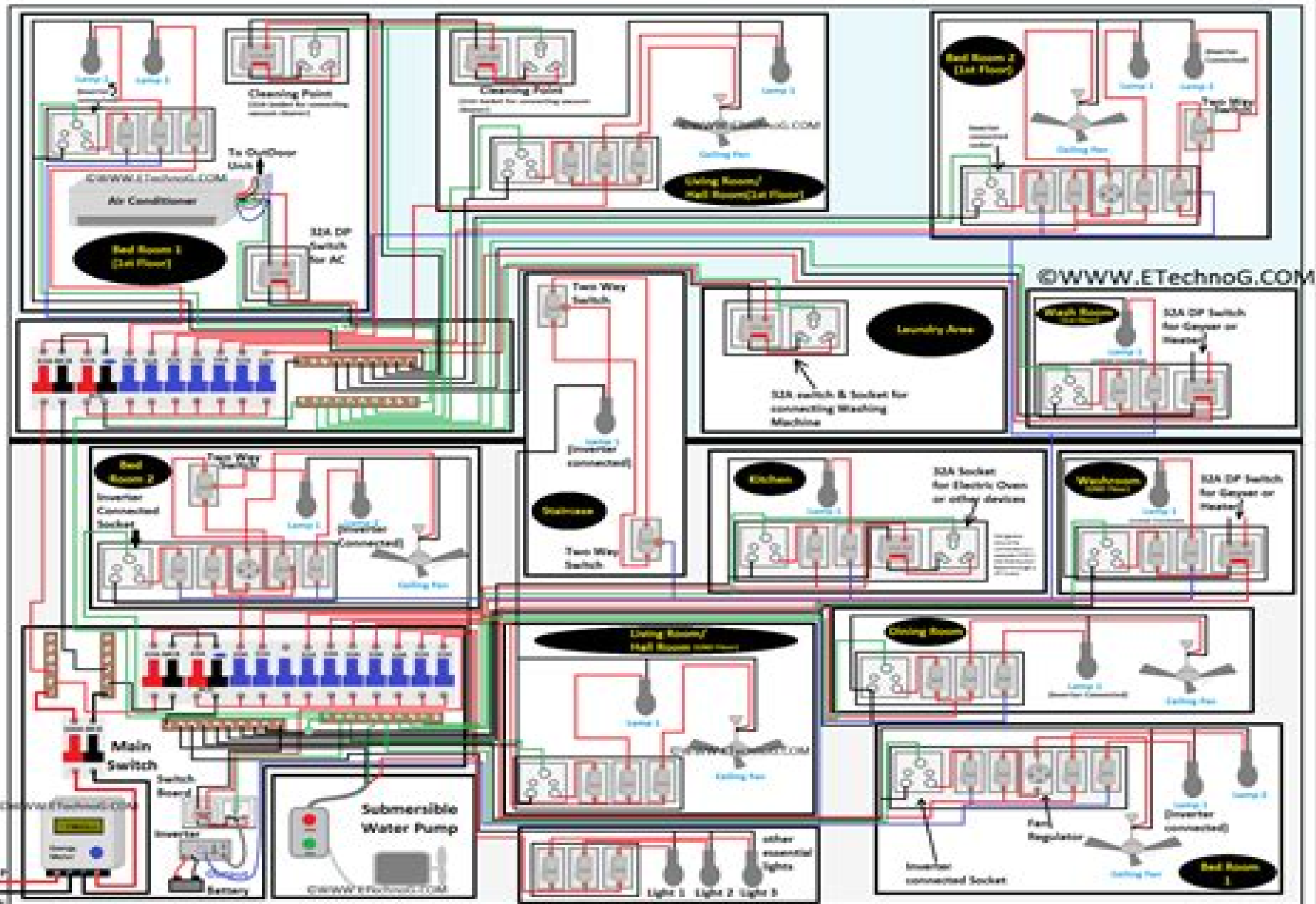
Complete House Wiring Diagram and Connection (Electrical Wiring for a two floor house)
