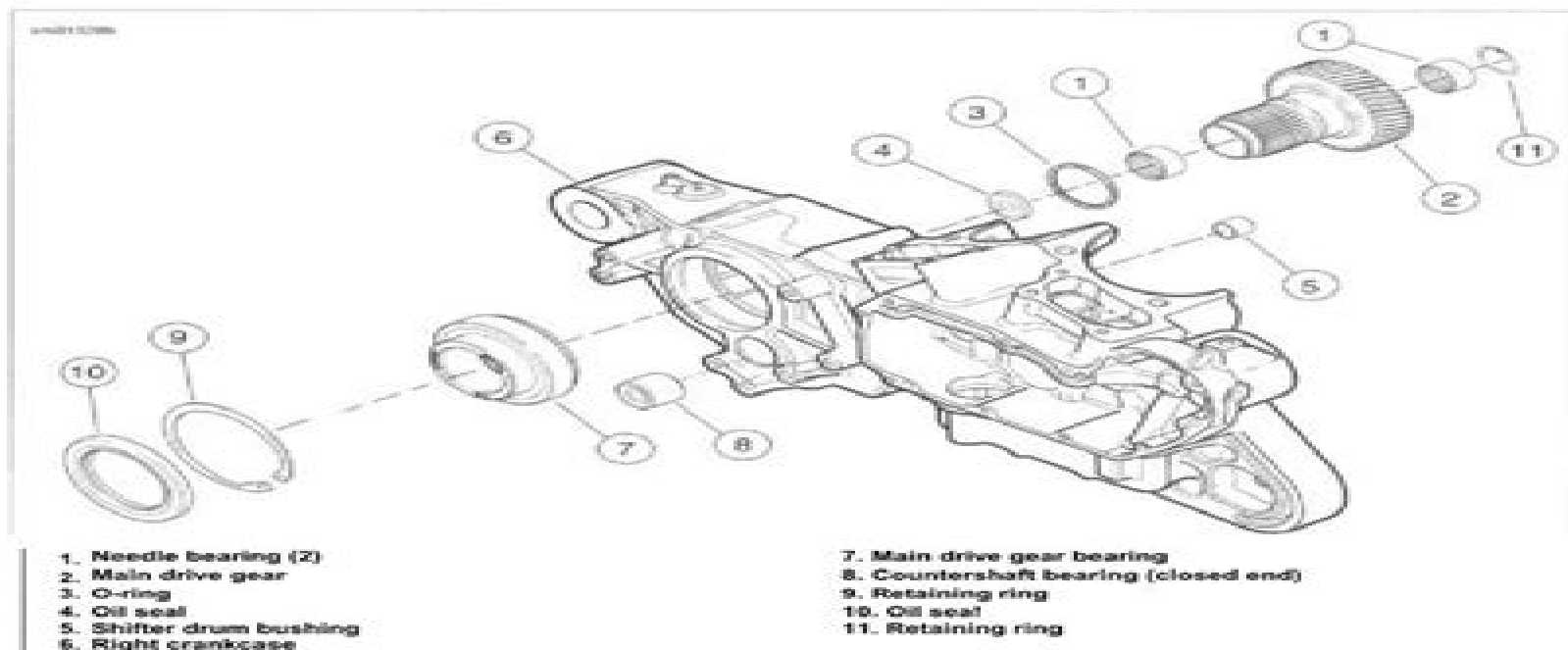
Figure 5-51. Main Drive Gear and Bearing Assembly
