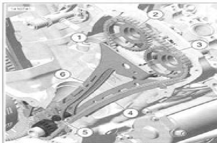
1. Timing chain 2. Intake sprocket 3. Exhaust sprocket 4. Fixed chain guide assembly 5. Screw 6. Dynamic chain guide assembly
