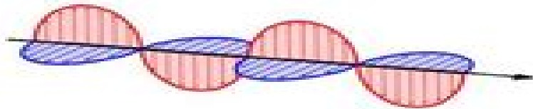
Electromagnetic Wave
