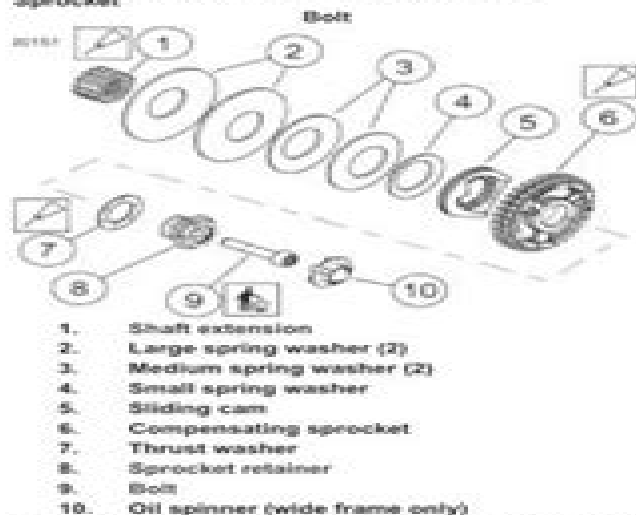
Figure 5-16. Engine Compensating Sprocket Assembly
