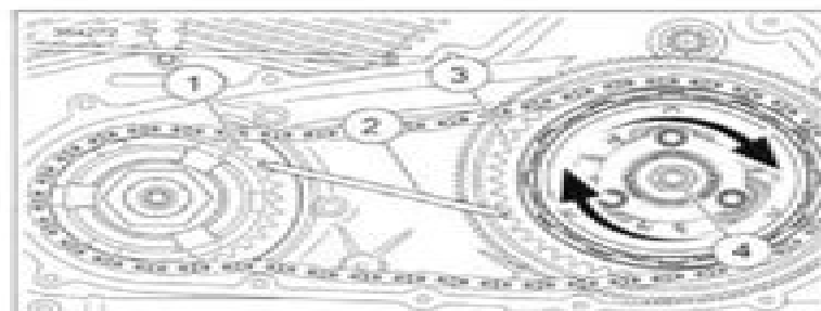
Figure 5-14. Removing Clutch Hub Mainshaft Nut
