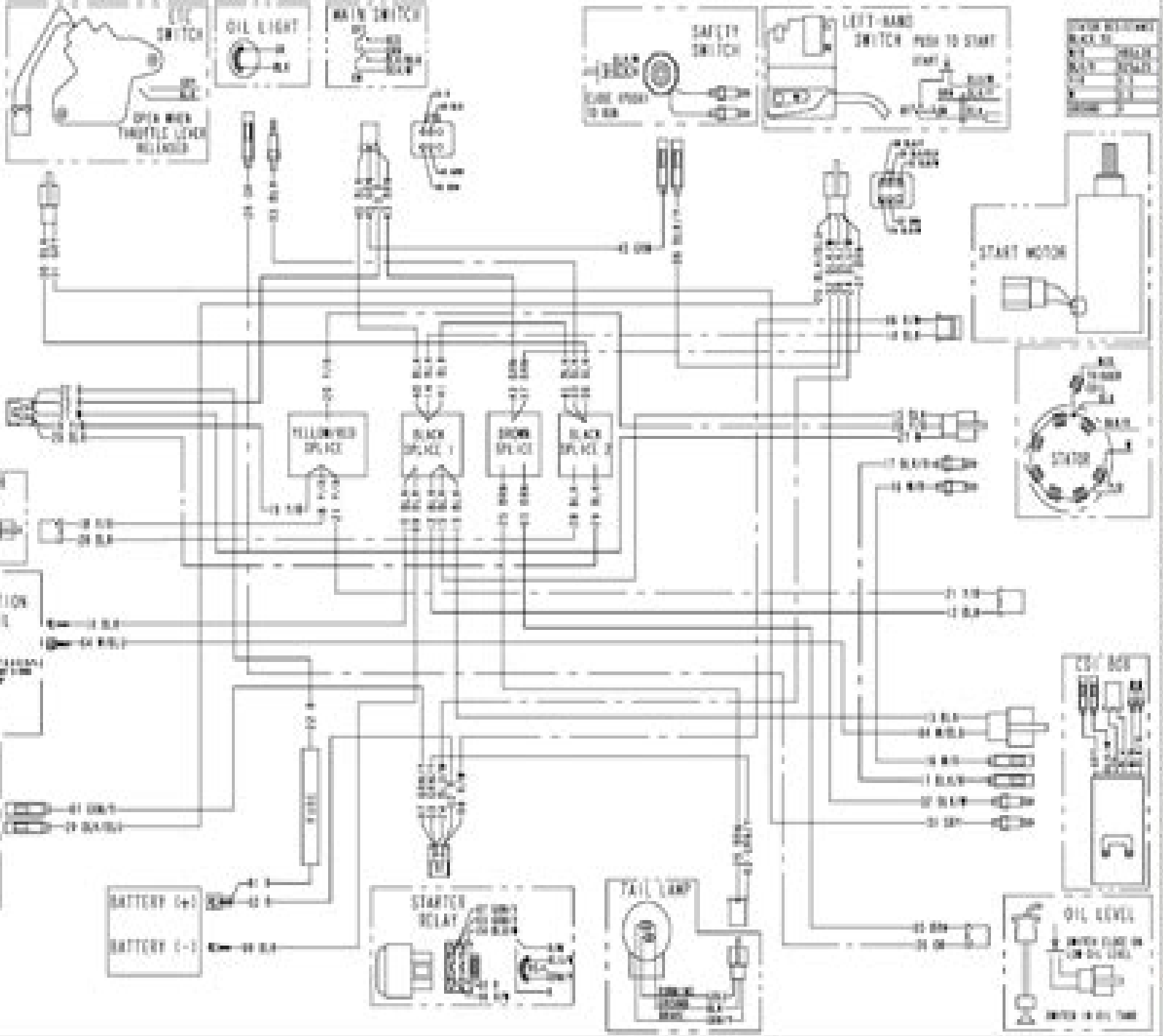
SCRAMBLER 90 / SPORTSMAN 90 / PREDATOR 90 WIRING DIAGRAM
