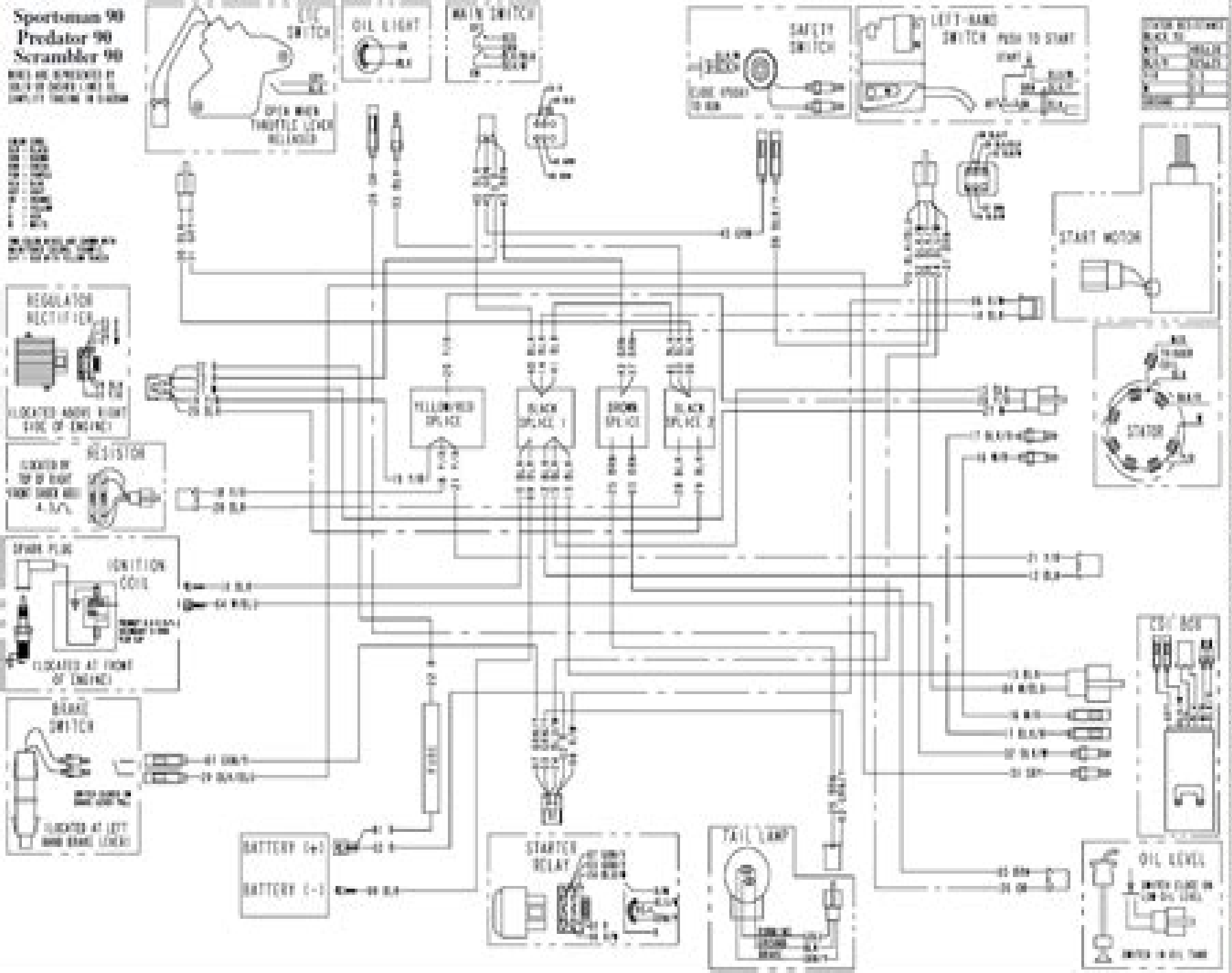
SCRAMBLER 90 / SPORTSMAN 90 / PREDATOR 90 WIRING DIAGRAM
