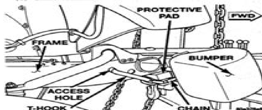
Fig. 3 T-Hook Attachment
