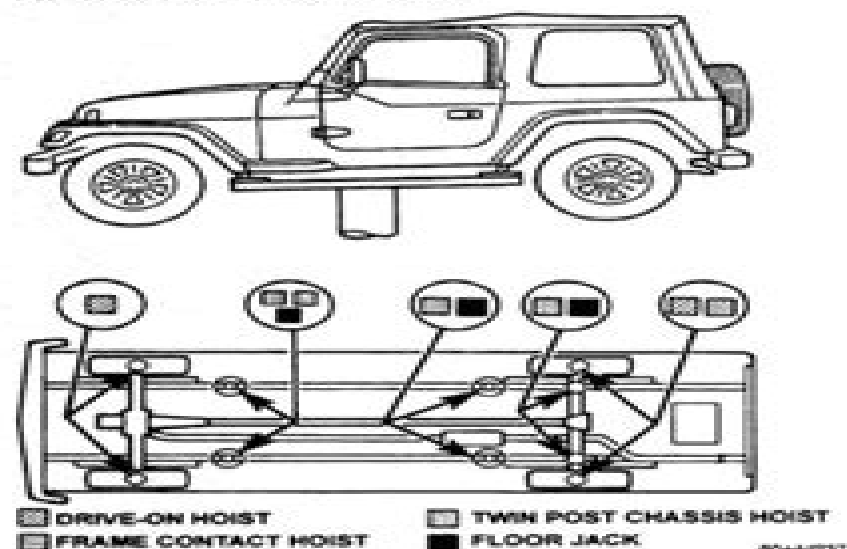
Fig. 5 Vehicle Lifting Locations
