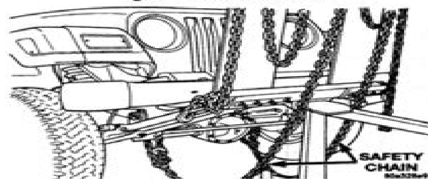
Fig. 4 Safety Chain Attachment
