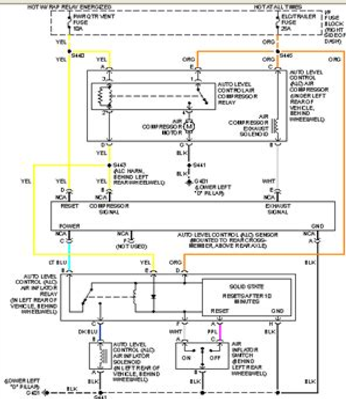
Fig. 14: Electronic Suspension Circuit, W/ Initiator
