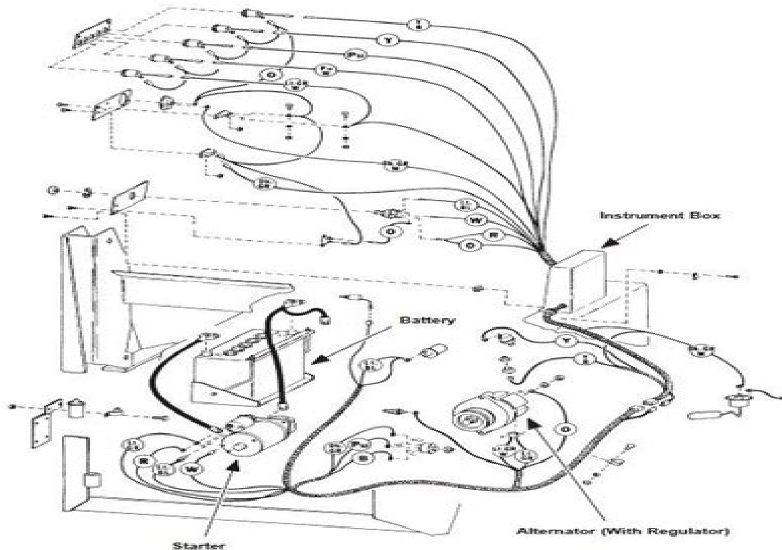
*Fig. 6-3 Electrical Circuitry (722)
