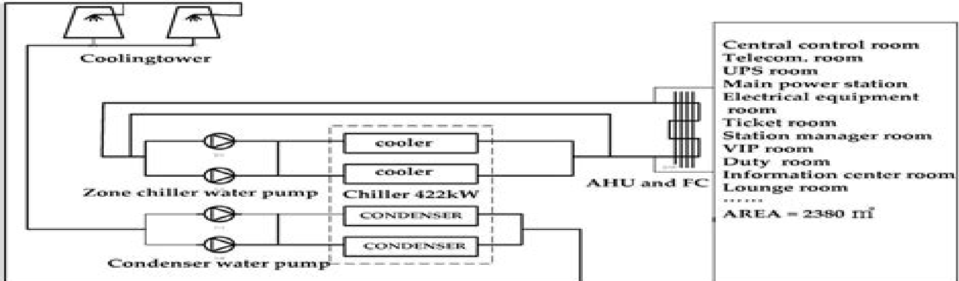
24 h supply air-conditioning system
