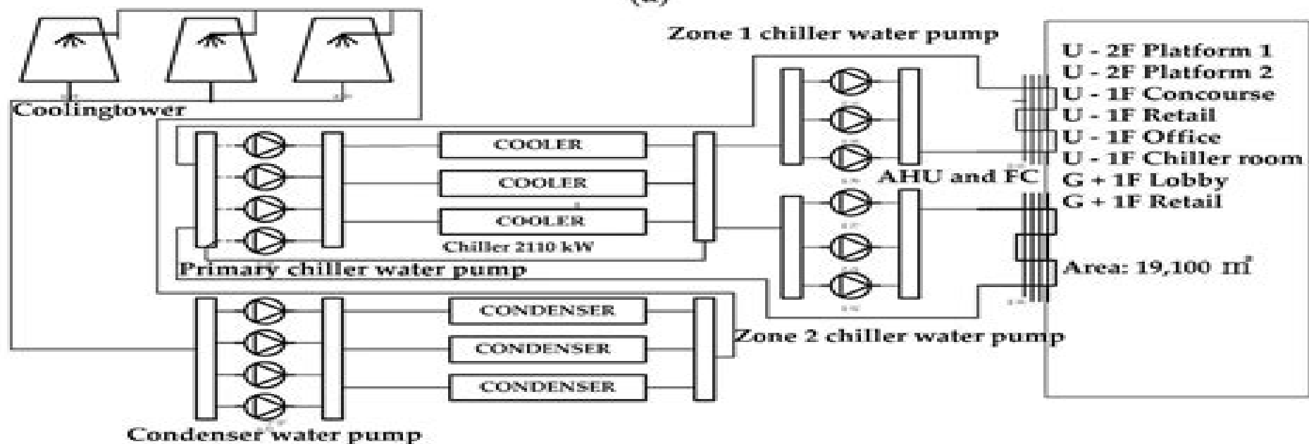
24 h supply air-conditioning system
