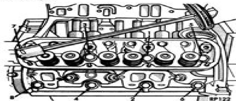
Fig. 5 Cylinder Head Bolt Tightening Sequence
