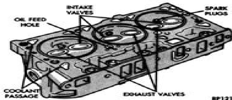
Fig. 4 Cylinder Head Assembly
